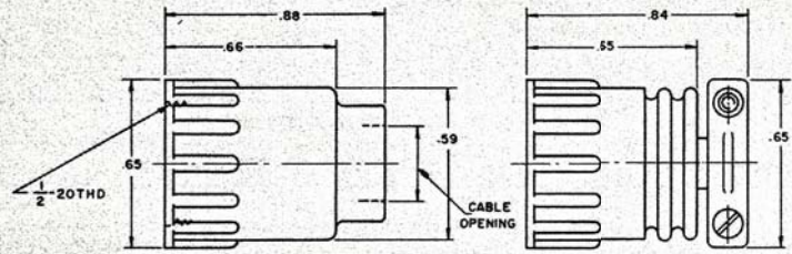
FIGS. 1 & 2 C18, 9/64 CABLE OPENING C38, 19/64 CABLE OPENING
