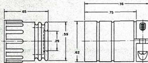
FIG. 6 C38G WITH GRIP
