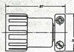
FIG. 4 C4/HC WITH CABLE CLAMP
