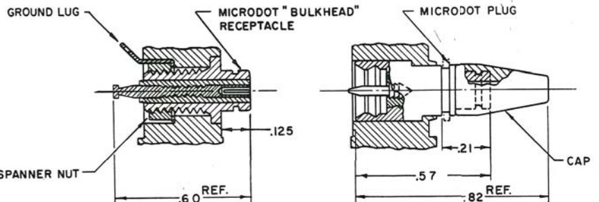
ENLARGED VIEW OF COAXIAL CONTACT
