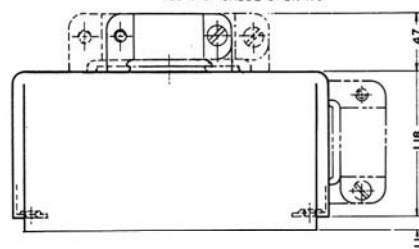
75 - 20H 75 - 20H - 1 75 - 20H2 (SHOWN IN PHANTOM)
